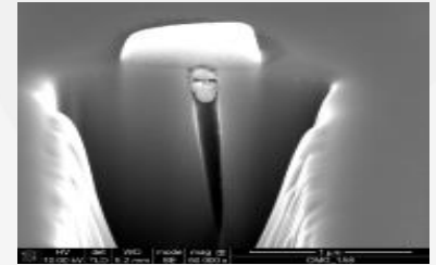
Defect Cross section AFM and SEM/FIB
